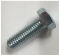
M8-1.25 x 35mm, Gr. 8.8 Bolt (12)
